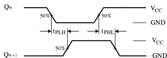
Figure 2. Switching Waveforms
