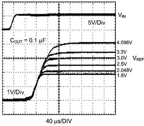
Start-Up Response
