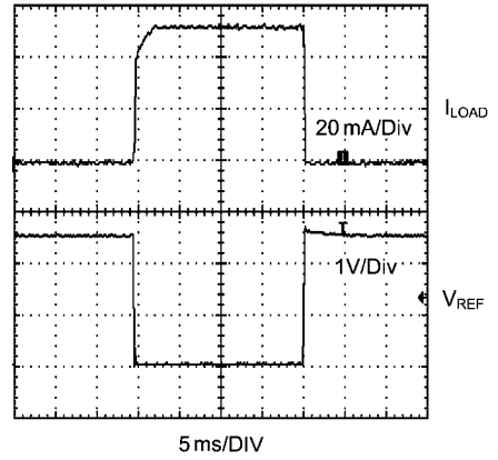
Short-Circuit Protection and Recovery
