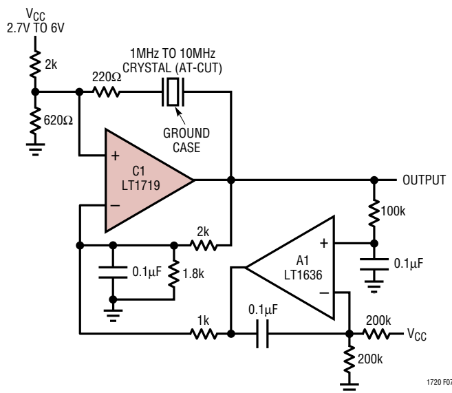
Figure 8. Crystal Oscillator with a Forced 50% Duty Cycle
