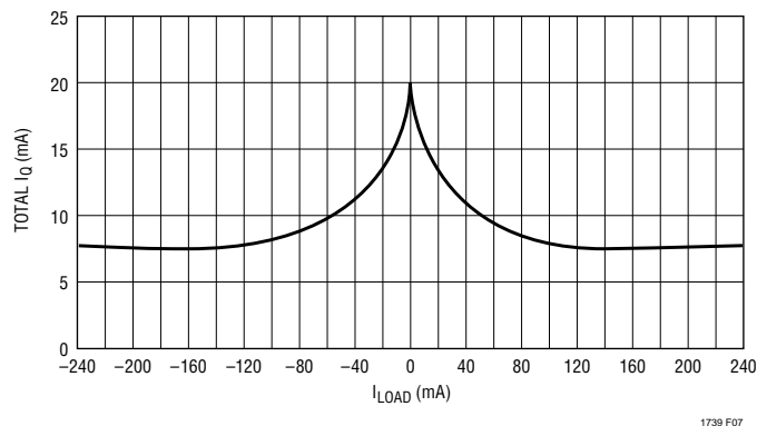
Figure 7. I_Q vs I_{LOAD}
