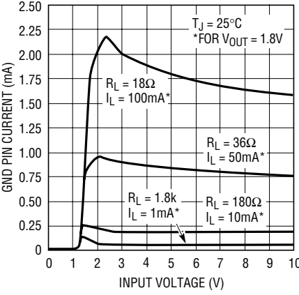
LT1761-1.8 GND Pin Current
