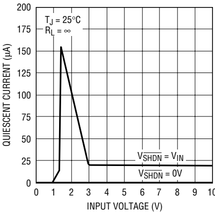
LT1761-3 Quiescent Current
