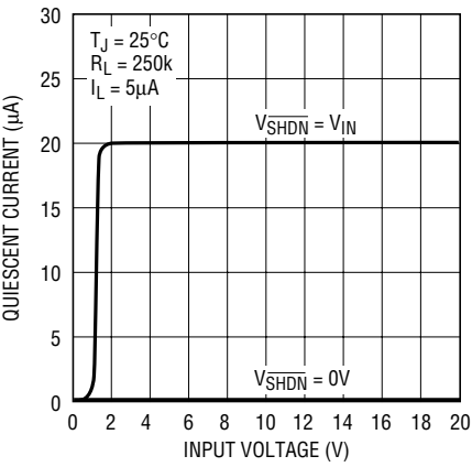
LT1761-BYP, LT1761-SD Quiescent Current
