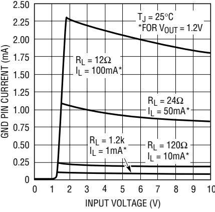
LT1761-1.2 GND Pin Current
