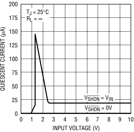
LT1761-2.5 Quiescent Current
