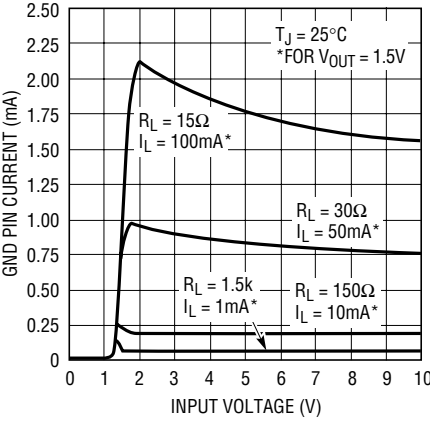
LT1761-1.5 GND Pin Current
