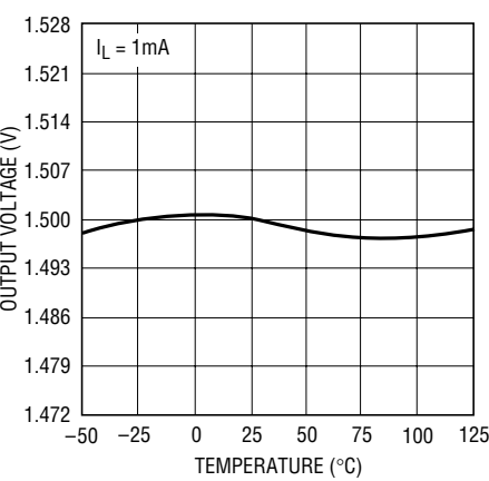
LT1761-1.5 Output Voltage
