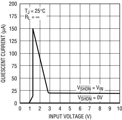
LT1761-2.8 Quiescent Current
