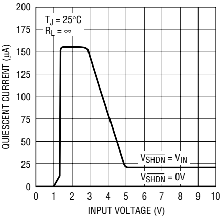
LT1761-5 Quiescent Current
