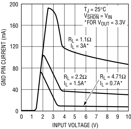
LT1764-3.3 GND Pin Current
