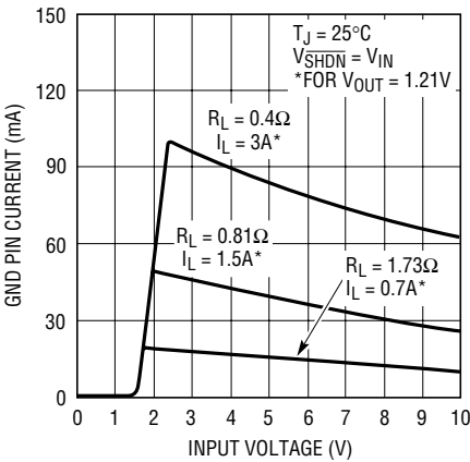
LT1764 GND Pin Current
