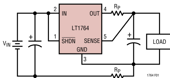
Figure 1. Kelvin Sense Connection
