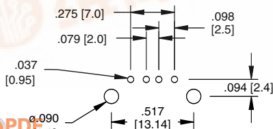
Recommended PCB Layout (Bottom View)
