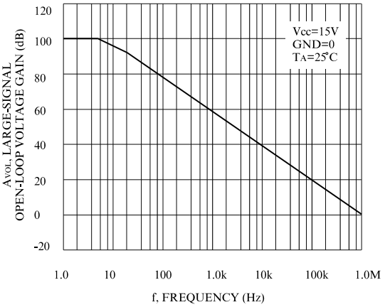
Figure 2. Open-Loop Frequency
