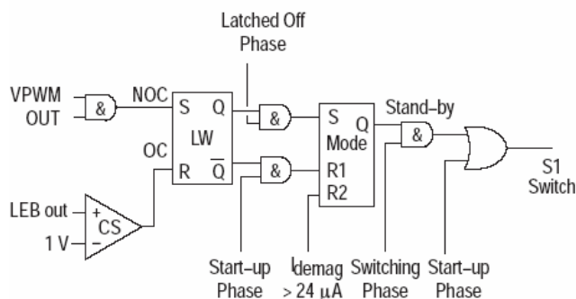
Figure 8. Transition Logic
