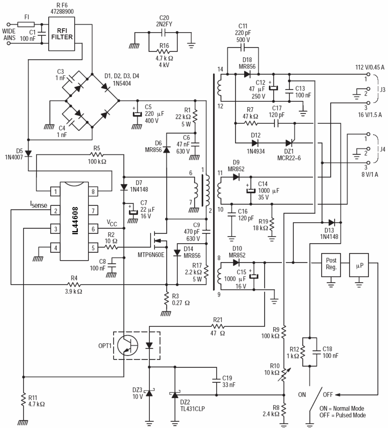
Figure 12. Typical Application
