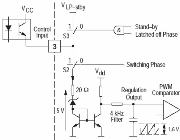
Figure 2. Regulator
