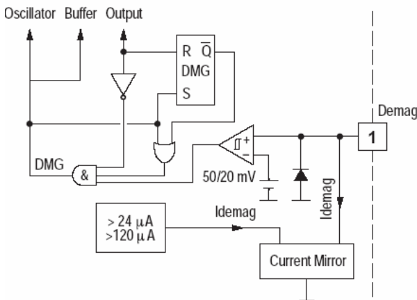
Figure 4. Demagnetization Block
