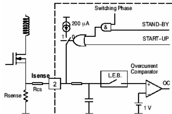
Figure 3. Current Sense
