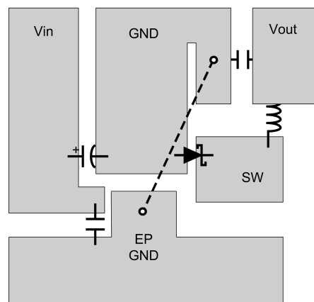
FIGURE 11. Example PCB Layout
