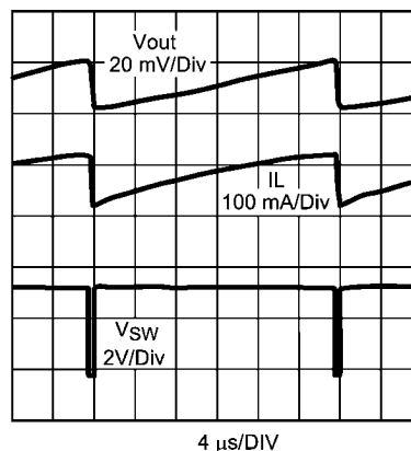
FIGURE 6. Off-pulse Skipping Waveforms Vin = 3.5V, Vnom = 3.3V, f_{\text{nom}} = 305\text{kHz}
