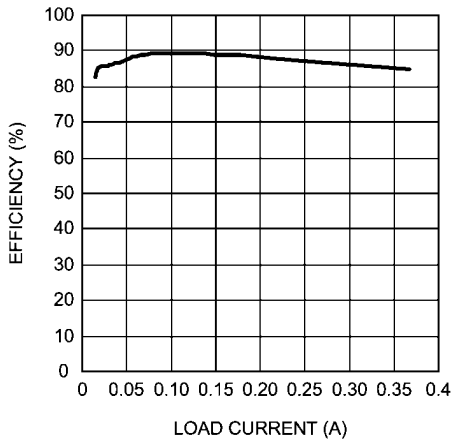
Boost Converter Efficiency vs I LOAD(DC) V_{DD} = 3V, PV_1 = 4.8V
