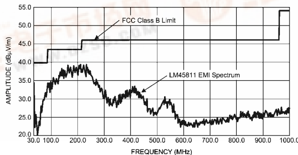
FIGURE 1. LM48511 RF Emissions — 3 inch cable
