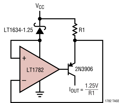
Current Source
