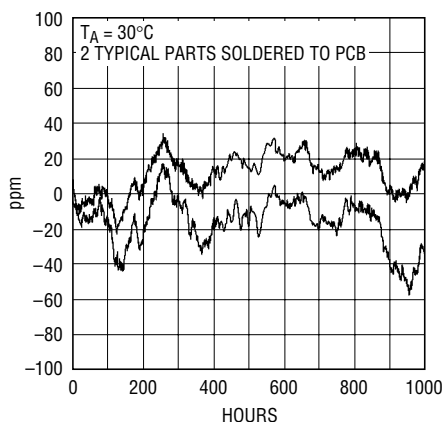
Long-Term Drift
