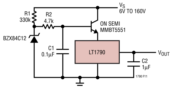
Figure 11. Extended Supply Range Reference
