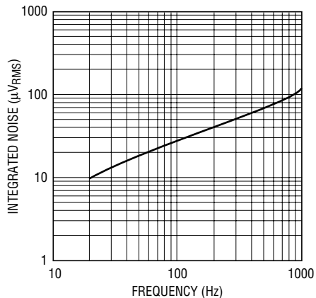
Intergrated Noise 10Hz to 1kHz
