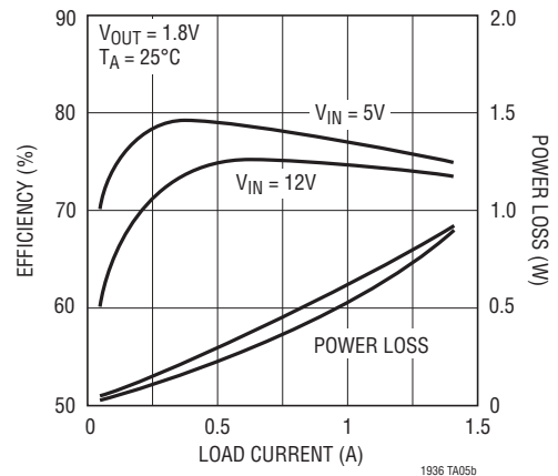
Efficiency, 1.8V Output
