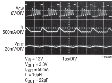
Switching Waveforms, Discontinuous Mode
