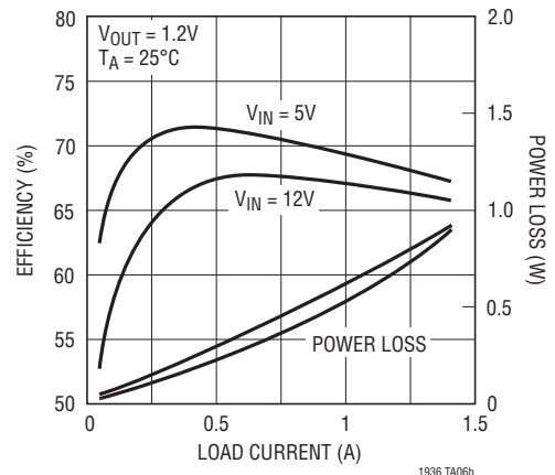
Efficiency, 1.2V Output
