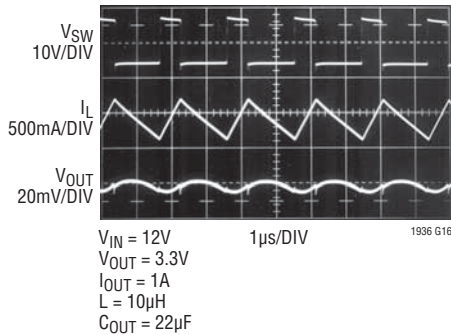
Switching Waveforms
