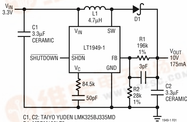
Figure 1. 3.3V to 10V/175mA DC/DC Converter
