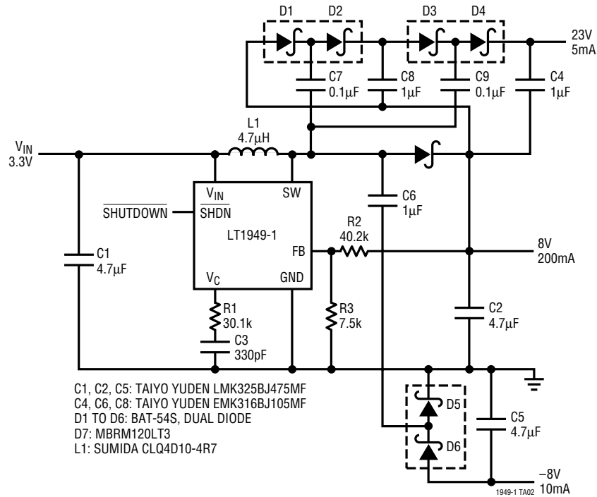
Low Profile Triple Output LCD Bias Generator
