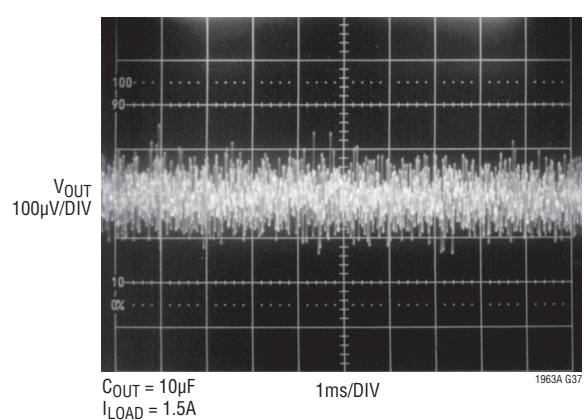
LT1963A-3.3 10Hz to 100kHz Output Noise
