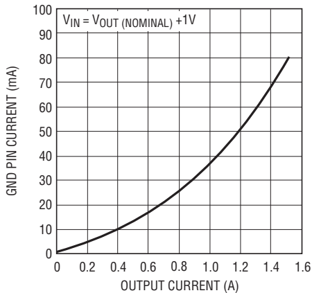
GND Pin Current vs I_{\text{LOAD}}
