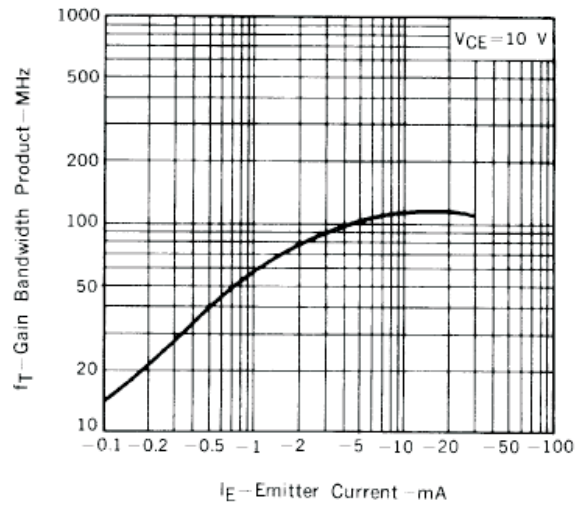
Fig.7 Gain Bandwidth Product vs. Emitter Current
