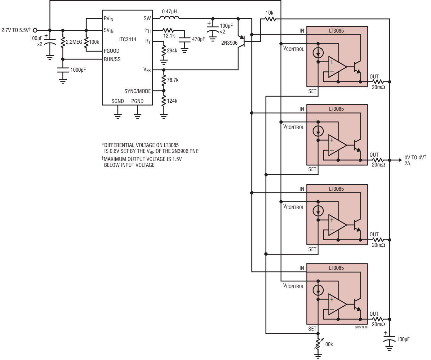
Low Voltage, High Current Adjustable High Efficiency Regulator*
