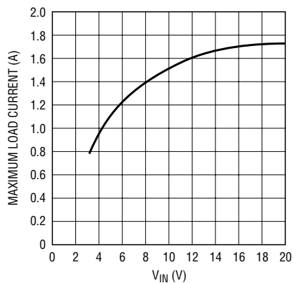
Maximum Load Current Increases with Input Voltage
