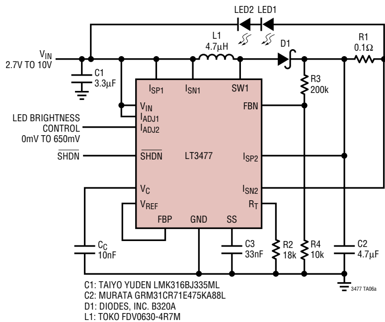
Buck-Boost Mode LED Driver
