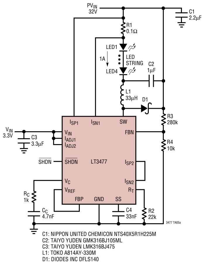
1A Buck Mode High Current LED Driver
