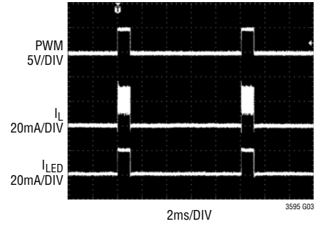
PWM Dimming Waveforms (10:1)
