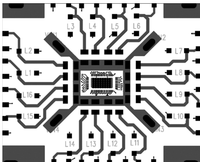
Figure 4. PCB Layer 1
