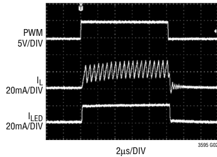
PWM Dimming Waveforms (1000:1)
