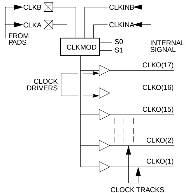
Figure 6 • Clock Networks
