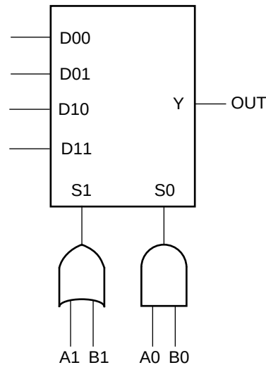
Figure 2 • C-Module Diagram
