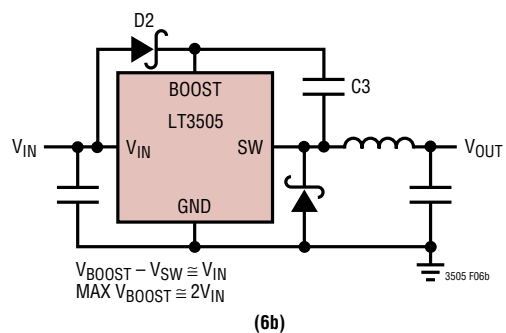
Figure 6. Two Circuits for Generating the Boost Voltage
