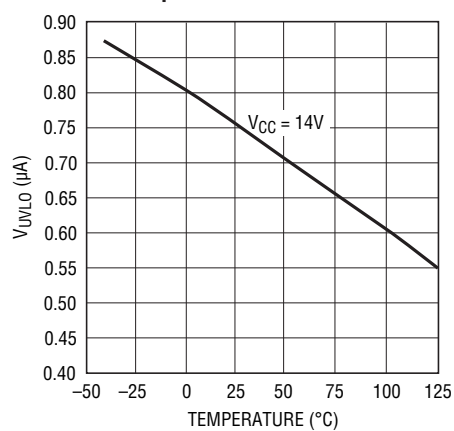
UVLO Shutdown Threshold vs Temperature
