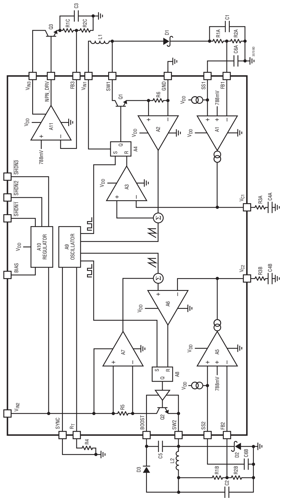
Figure 1. Block Diagram
