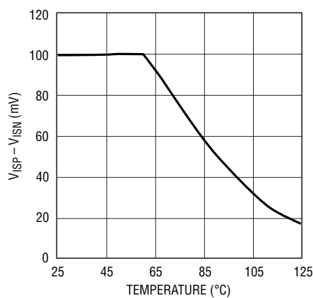
V ISP -V ISN vs Temperature for NTC Resistor Divider
