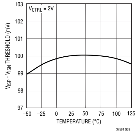
V_{ISP} - V_{ISN} Threshold vs Temperature
