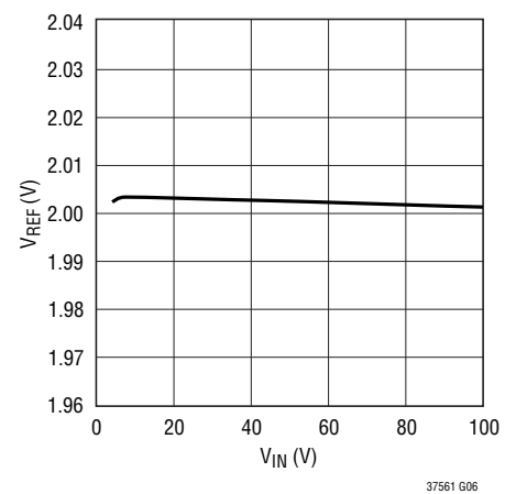
V_{REF} Voltage vs V_{IN}
