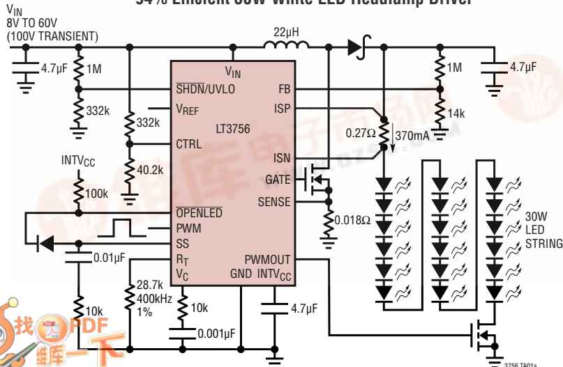
94% Efficient 30W White LED Headlamp Driver
