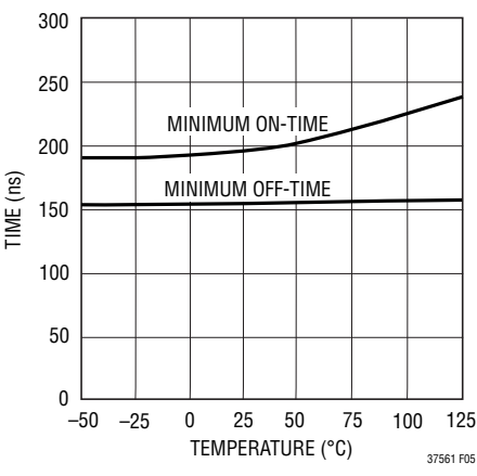
Figure 5. Typical Minimum On and Off Pulse Width vs Temperature
