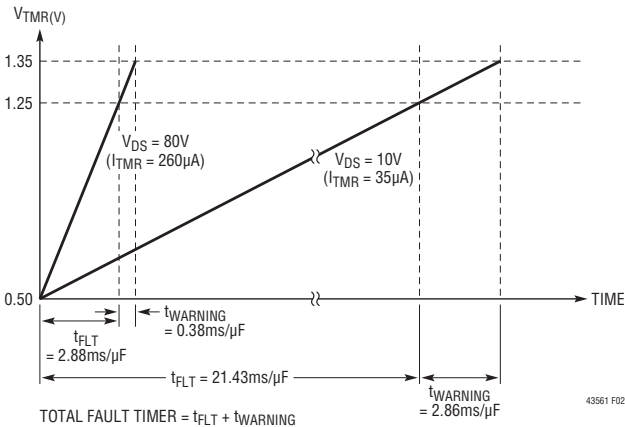
Figure 2. Overcurrent Fault Timer Current
