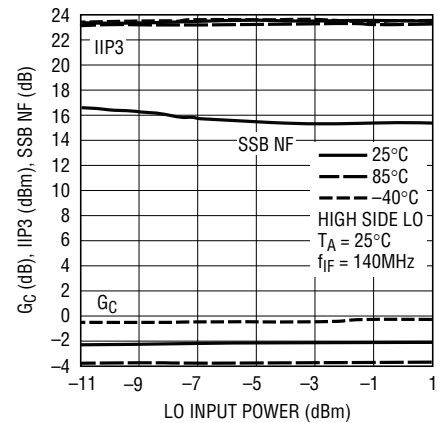
Conv Gain, IIP3 and SSB NF vs LO Input Power (RF = 450MHz)
