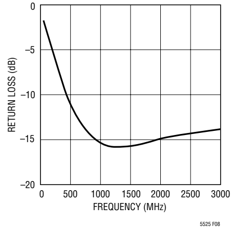
Figure 8. LO Input Return Loss
