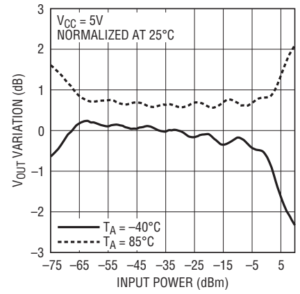
VOUT Variation vs Input Power at 40MHz
