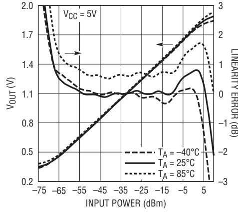
Output Voltage, Linearity Error vs Input Power at 40MHz
