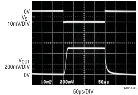
Step Response V_{SENSE} = 0\text{V to } 10\text{mV}, V_S^+ = 0\text{V}
