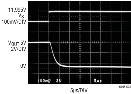
Step Response V_{SENSE} = 100\text{mV to } 5\text{mV}
