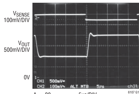
Step Response 50mV to 100mV ( R_{IN} = 500\Omega )
