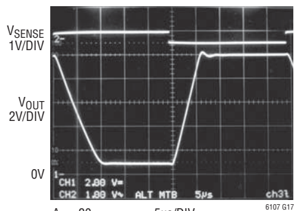
Step Response 50mV to 500mV ( R_{IN} = 500\Omega )
