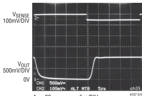
Step Response 0mV to 50mV ( R_{IN} = 500\Omega )
