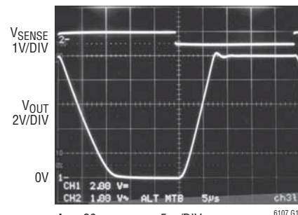
Step Response 0mV to 500mV ( R_{IN} = 500\Omega )
