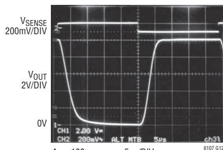
Step Response 0mV to 100mV ( R_{IN} = 100\Omega )
