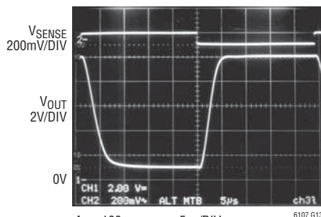
Step Response 10mV to 100mV ( R_{IN} = 100\Omega )
