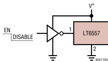
(3b) CMOS Gate with Shared Supply
