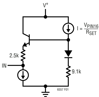
Figure 1. Simplified Programmable Input Bias Circuit Diagram
