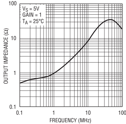
Output Impedance
