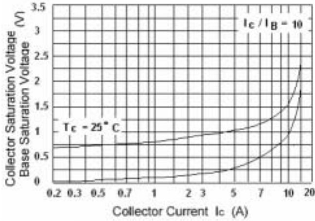
Fig.3 Base-Emmitter Saturation Voltage Collector-Emmitter Saturation Voltage
