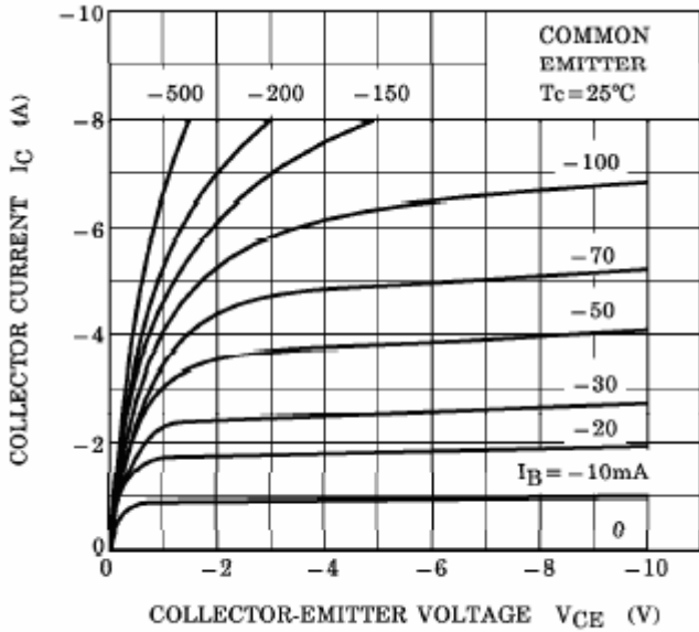
Fig.3 Static Characteristic
