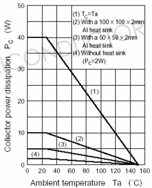
Fig.4 Power Derating
