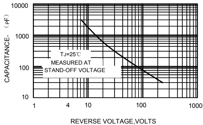
FIG.2-TYPICAL JUNCTION CAPACITANCE
