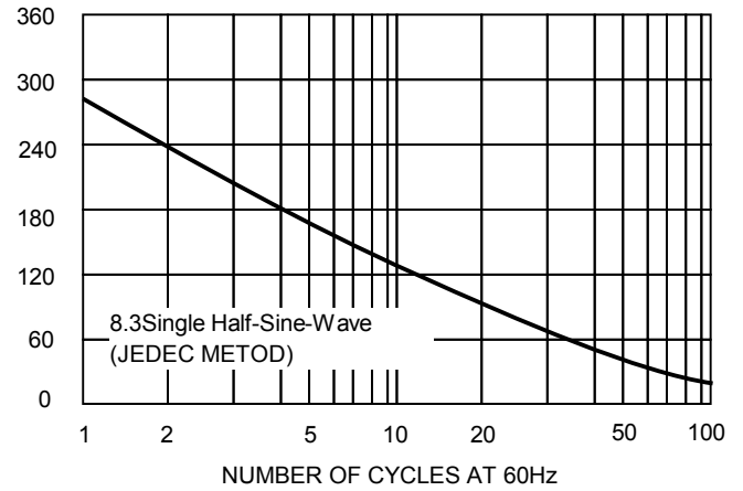
FIG.2-MAXIMUM NON-REPETITIVE SURGE
