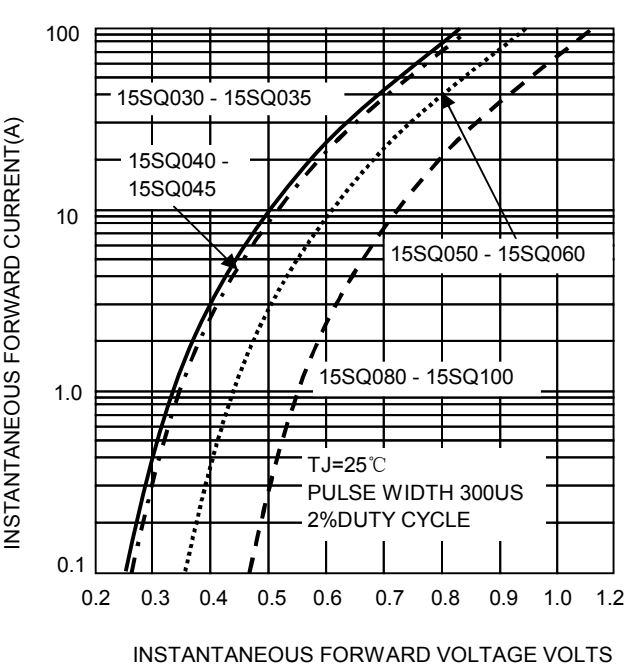
FIG.4-TYPICAL FORWARD CHARACTERISTICS
