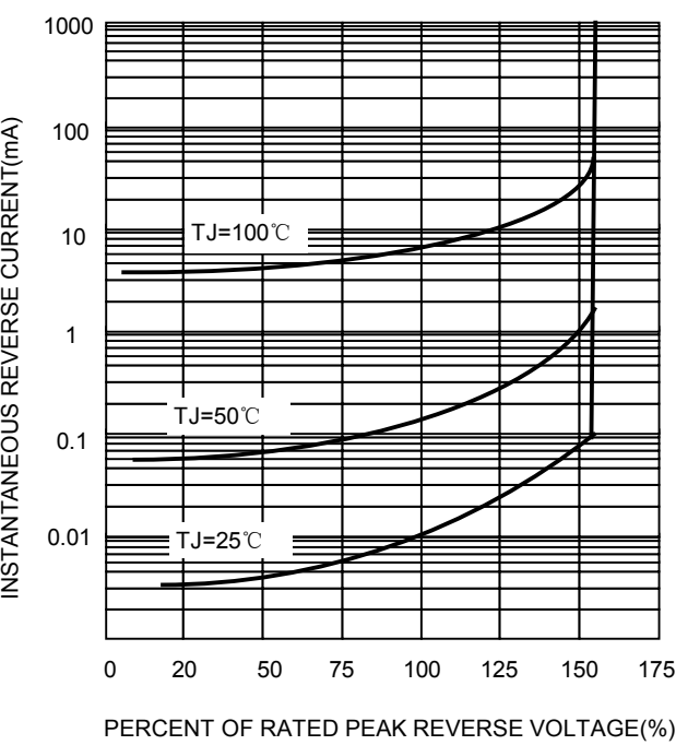
FIG.3-TYPICAL REVERSE CHARACTERISTICS
