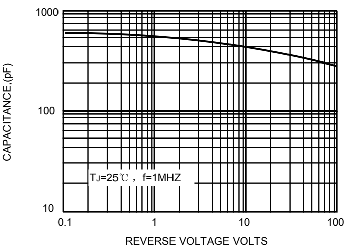
FIG.5-TYPICAL JUNCTION CAPACITANCE
