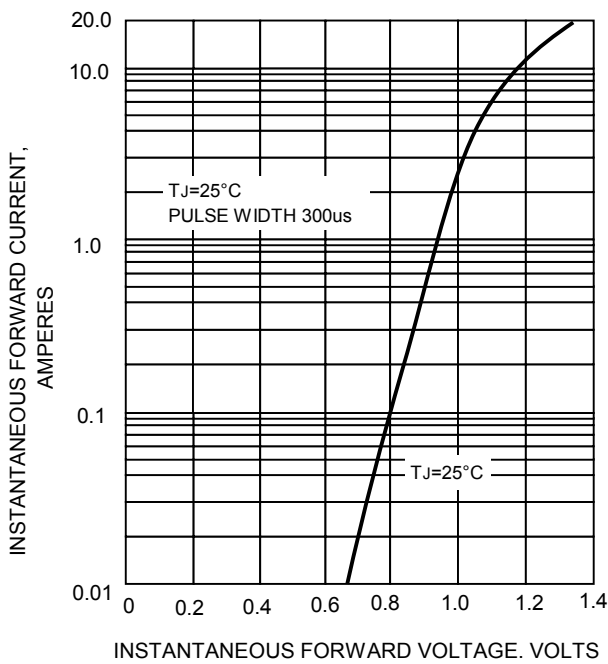
FIG.2-TYPICAL FORWARD CHARACTERISTICS
