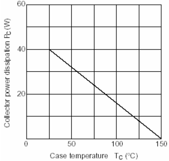
Fig.4 Power Derating
