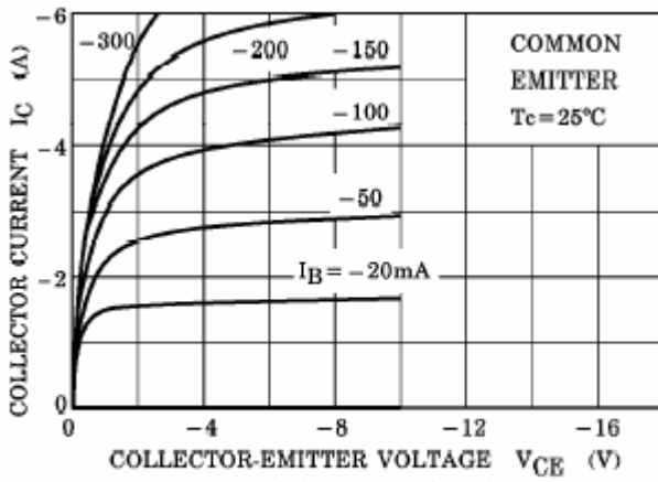
Fig.3 Static Characteristic
