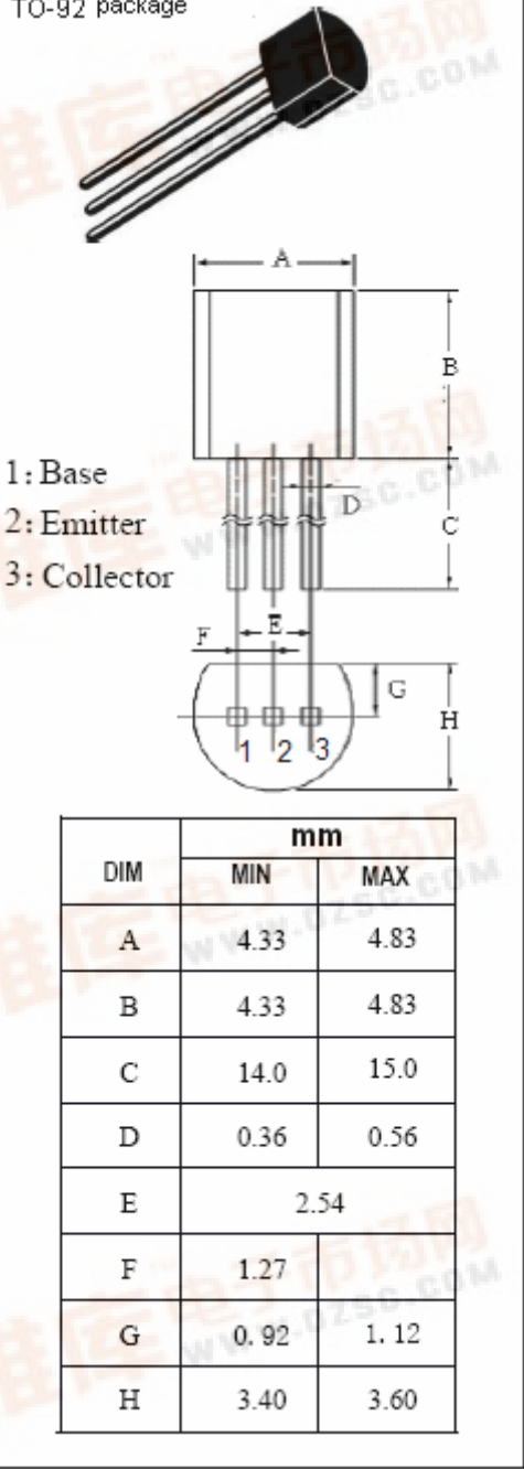
TO-92 package
