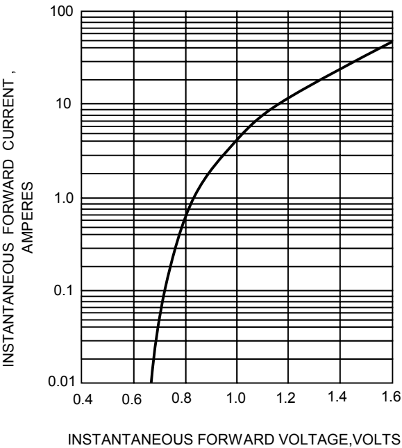
FIG.3-TYPICAL FORWARD CHARACTERISTICS
