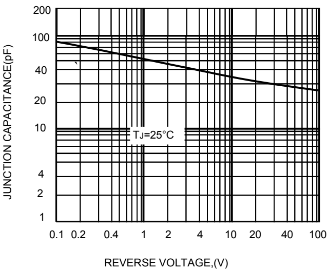
FIG.5-TYPICAL JUNCTION CAPACITANCE
