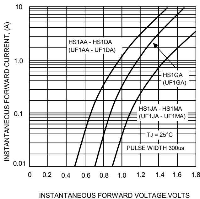
FIG.4-TYPICAL FORWARD CHARACTERISTICS
