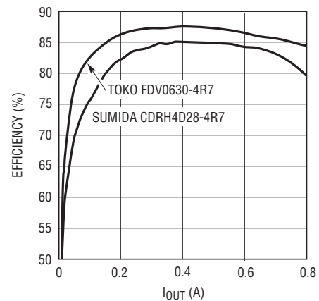
Figure 1. Efficiency vs Inductor Size
