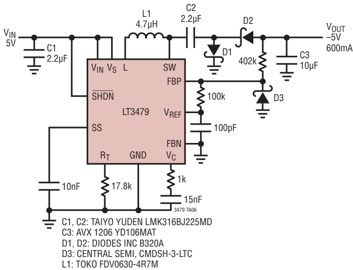
5V to -5V/600mA Inverting DC/DC Converter
