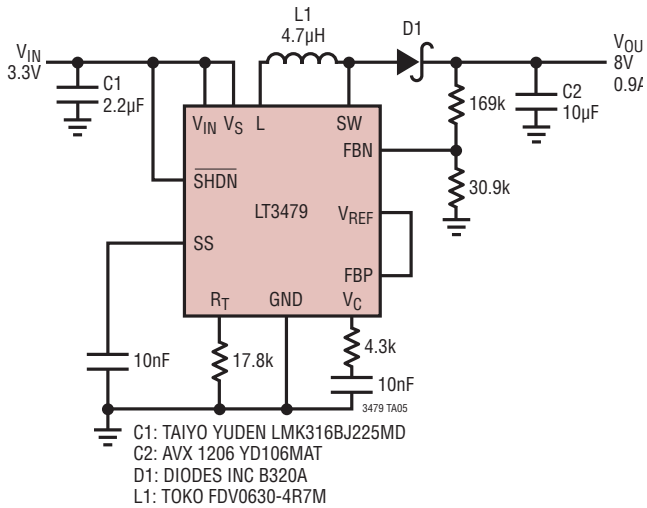
3.3V to 8V/900mA Boost Converter
