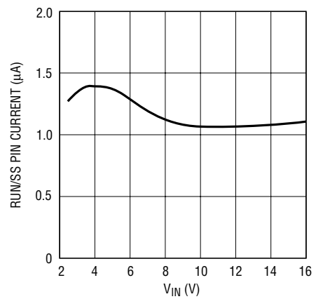
RUN/SS Pin Current vs V IN in Shutdown
