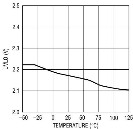
UVLO Voltage
