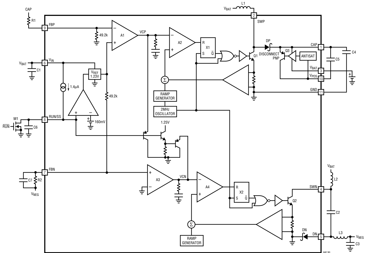
Figure 1. Block Diagram
