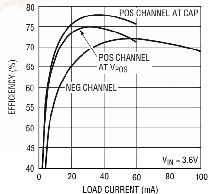
Conversion Efficiency
