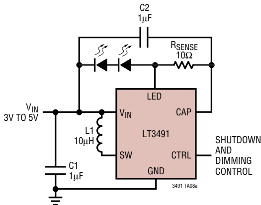
Li-Ion Driver for Two White LEDs
