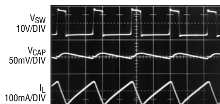
Switching Waveform
