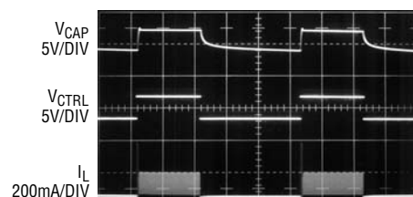
Transient Response
