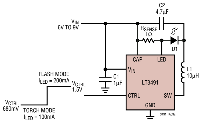
2-Cell Li-Ion Driver for Torch and Flash Mode LED Control
