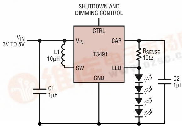
Li-Ion Driver for Four White LEDs
