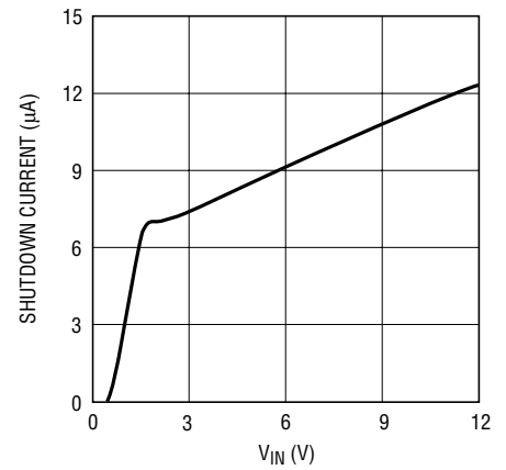
Shutdown Current (V CTRL = 0V)
