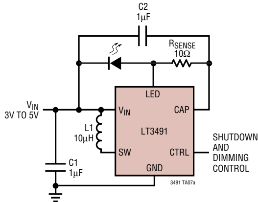
Li-Ion Driver for One White LED
